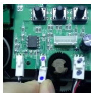
Figure 20: Connect the MAV Drive Cord to the Circuit Board
