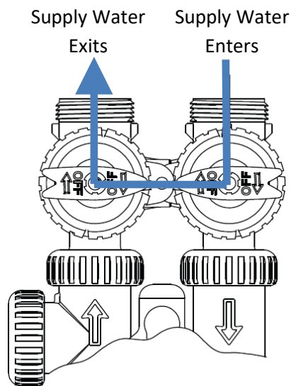
Figure 28: Bypass Operation
