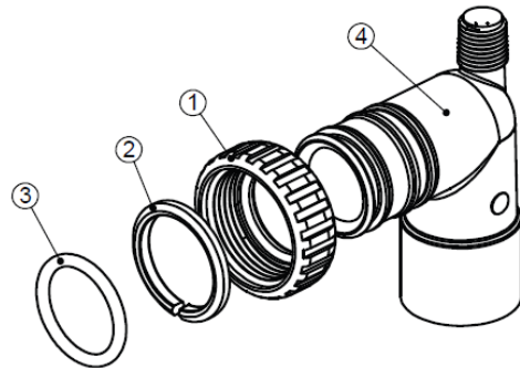
Order No: 12-0109-BR Description: DCS6 Fitting 3/4" Brass Sweat Assembly
