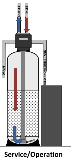
Figure 21: General Softener Operations
