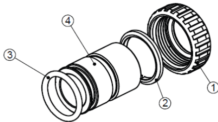
Order No: 12-0110-PL Description: DCS6 Fitting 1" Plastic Male NPT Assembly
