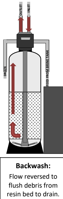
Figure 21: General Softener Operations
