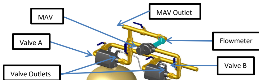
Figure 16: MAV connected to Valves
