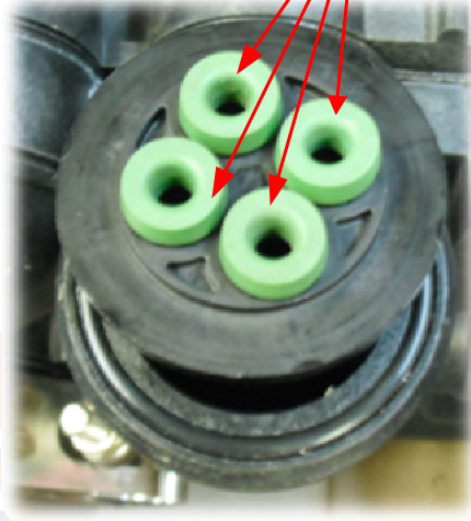
Drain Line Flow Control *Installed WRONG Buttons On Inside.
